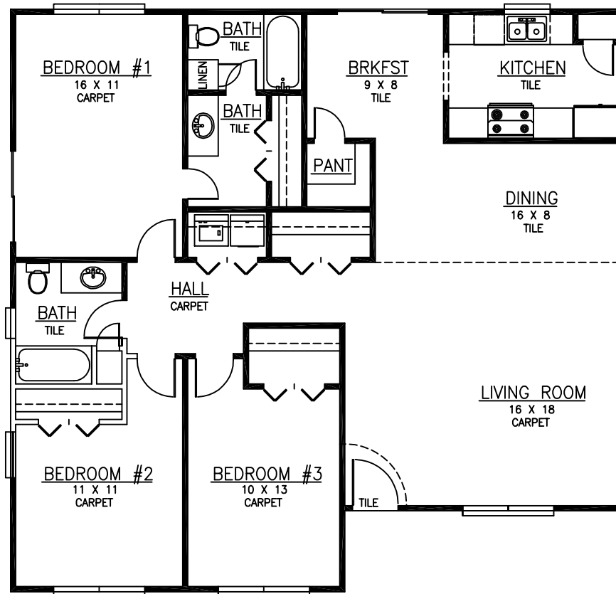
3 BEDROOM 2 BATH 1281 SQFT
