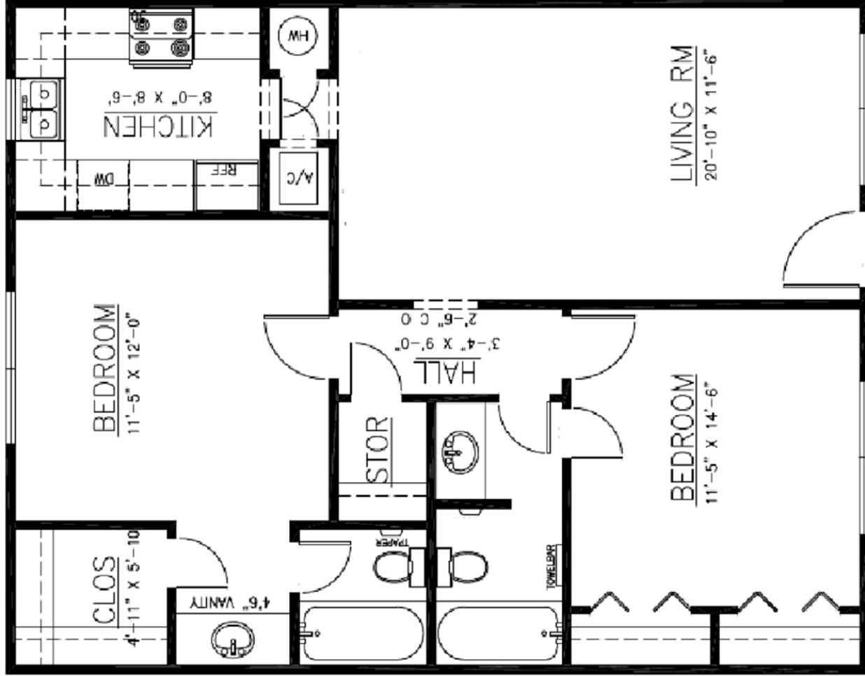
TWO BDRM 2 BATH UNIT
