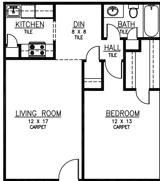
1 BEDROOM 1 BATH FLAT 650 SQFT
